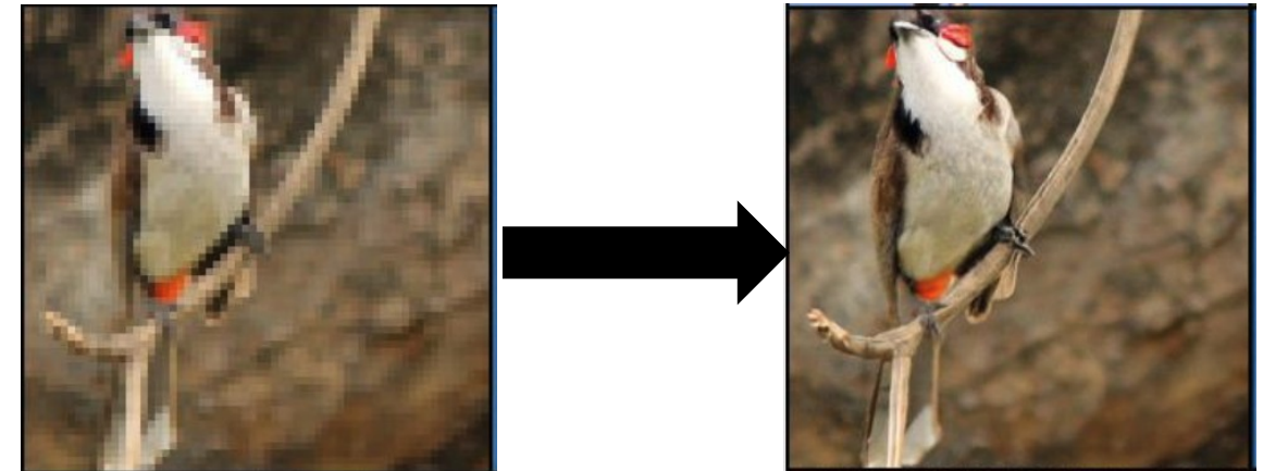
Super-resolution
